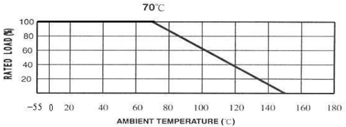
FIG.1 DERATING CURVE
